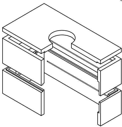
Two Piece Riser Option
