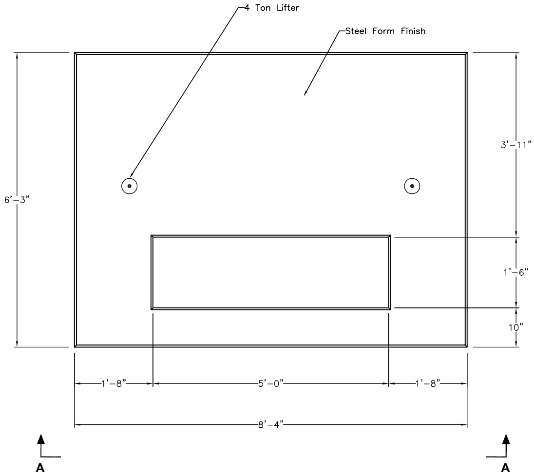
Plan View
