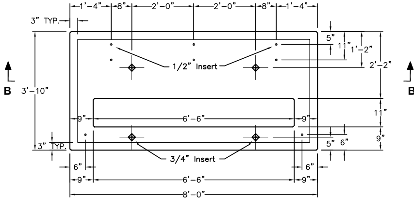
Pad / Plan View
