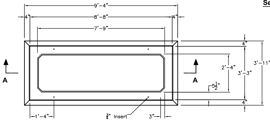
Pit / Plan View
